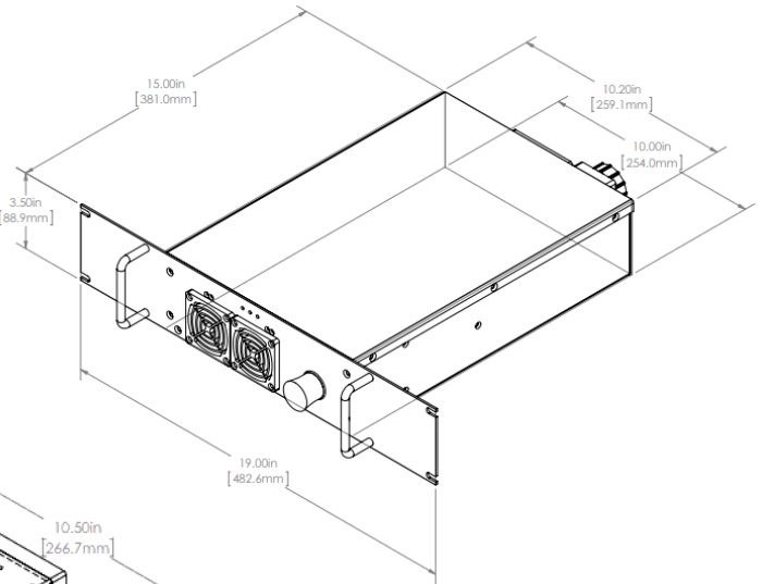
DM1 Power Supply
