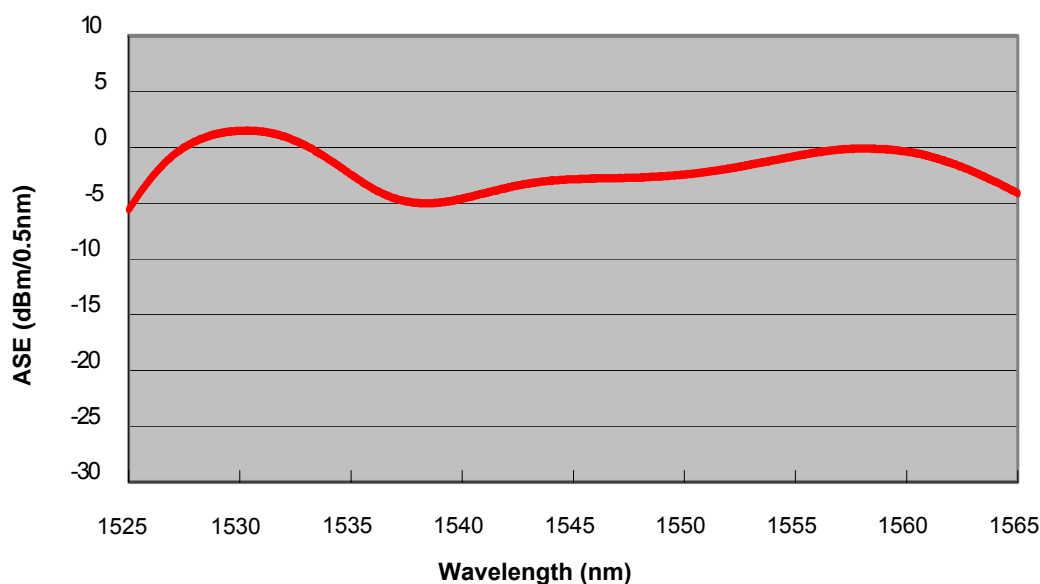
Typical Spectra:
