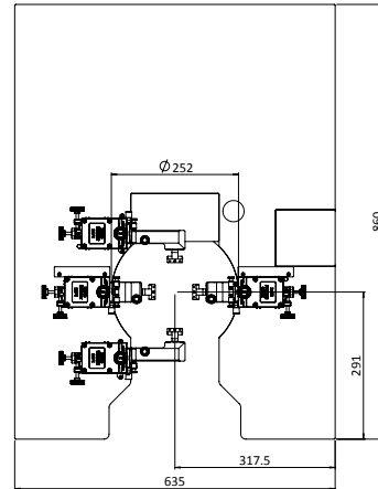
Probe platen design
